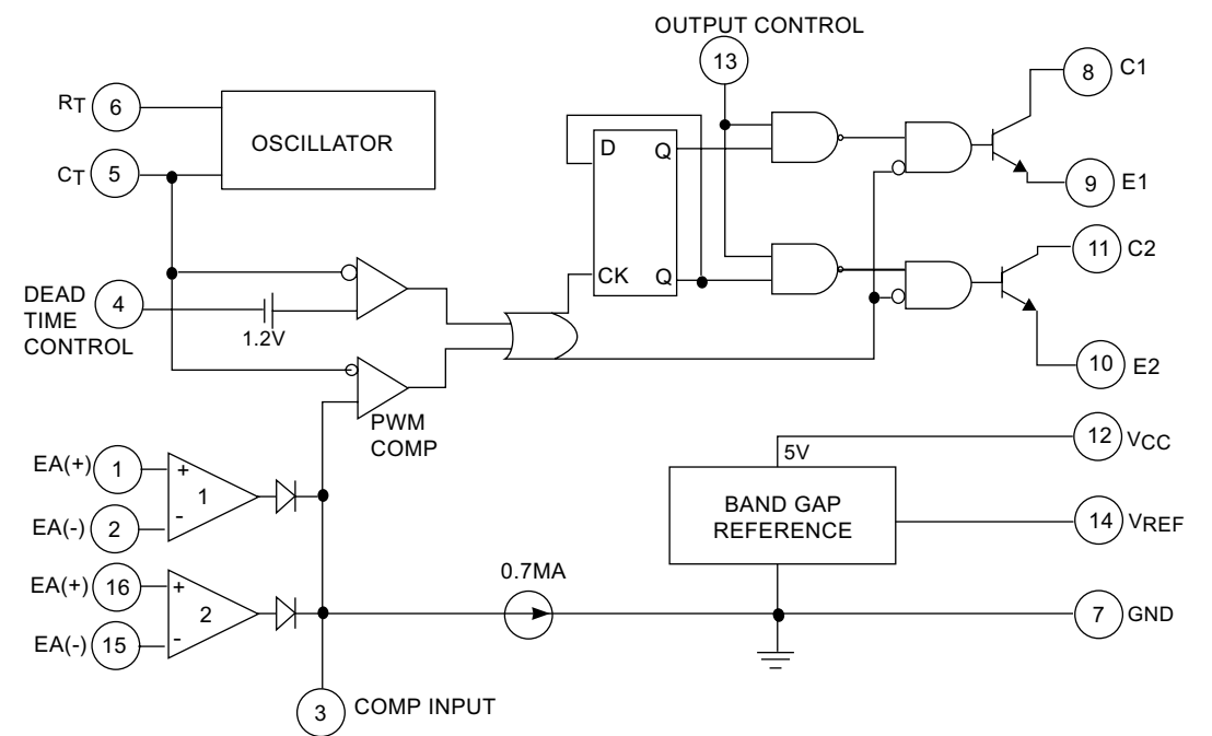
IC INTERNAL BLOCK DIAGRAM SMPS CONTROLLER - KA7500C
